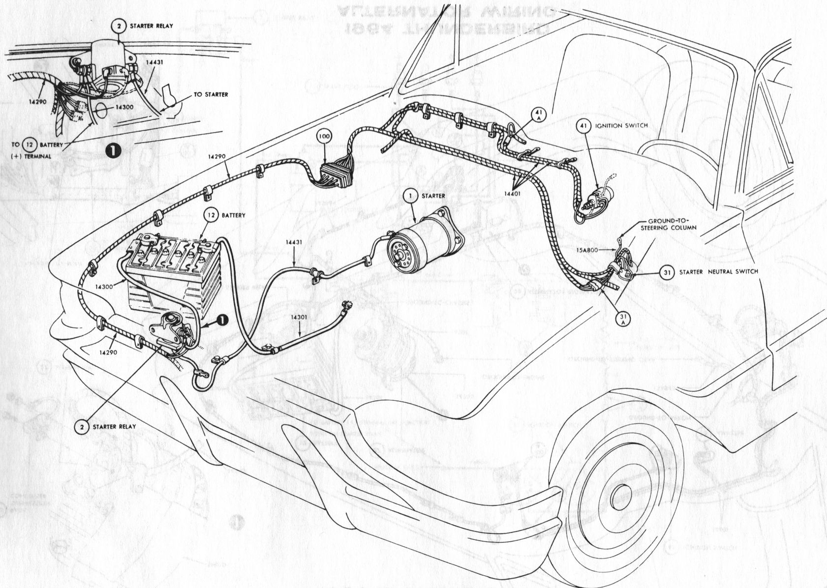
1964 THUNDERBIRD STARTER WIRING
