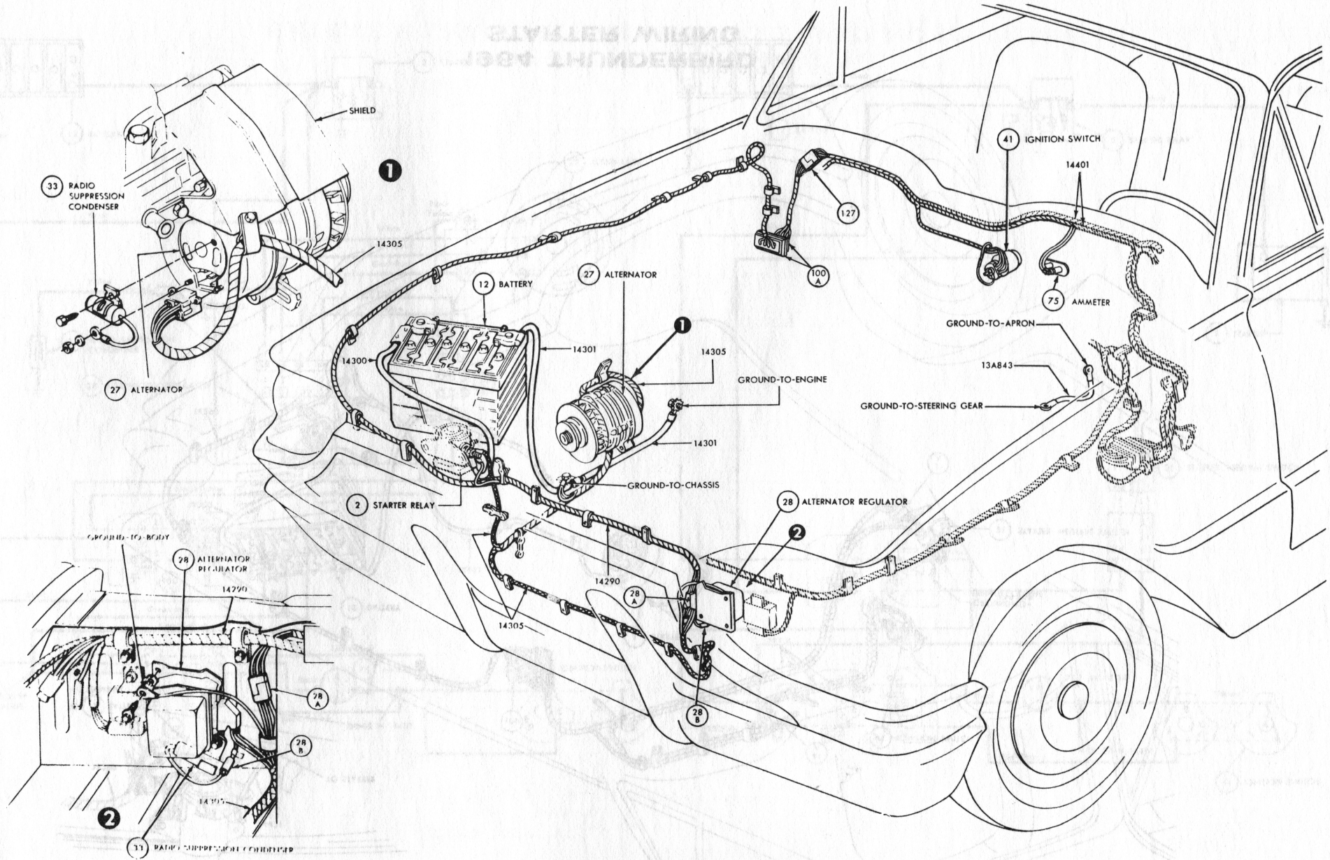
1964 THUNDERBIRD ALTERNATOR WIRING
