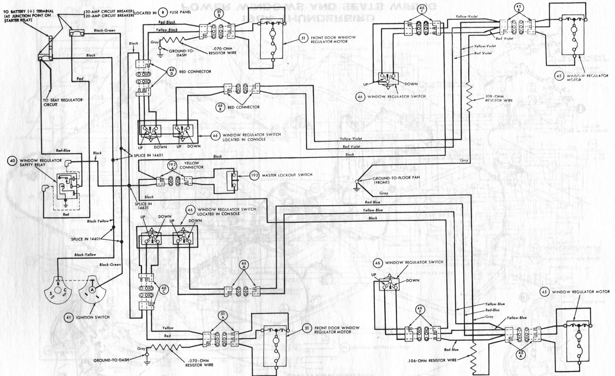
1964 THUNDERBIRD POWER WINDOWS SCHEMATIC
