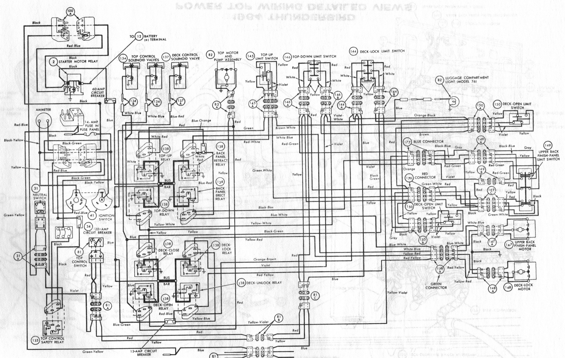
1964 THUNDERBIRD POWER TOP SCHEMATIC
