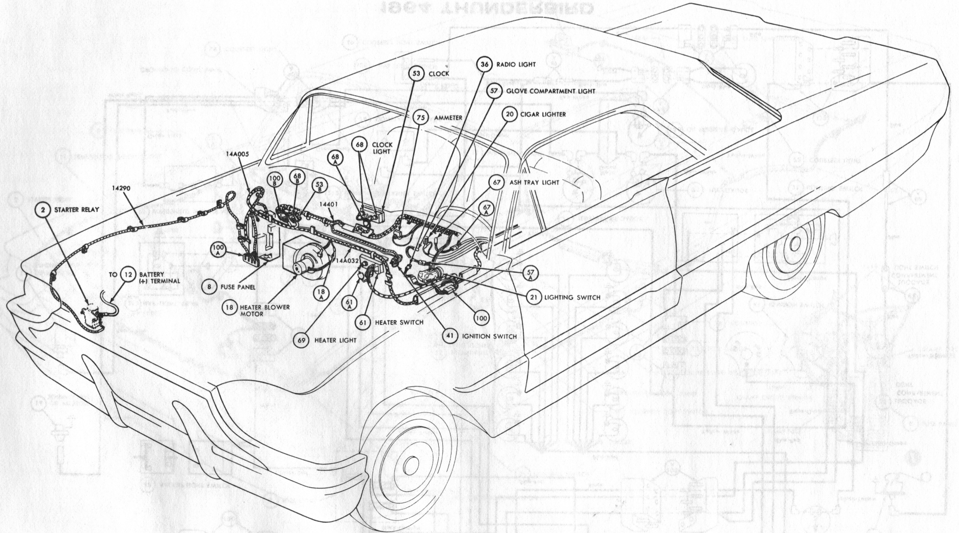
1964 THUNDERBIRD ACCESSORIES WIRING
