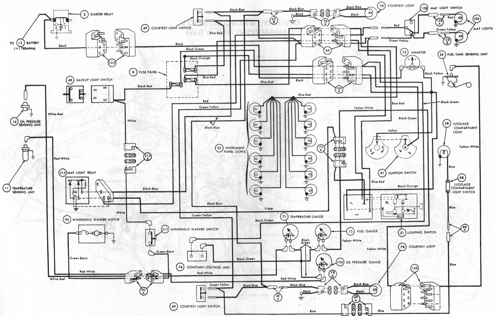
1964 THUNDERBIRD INTERIOR LIGHTING, WINDSHIELD WIPER AND GAUGE SCHEMATIC
