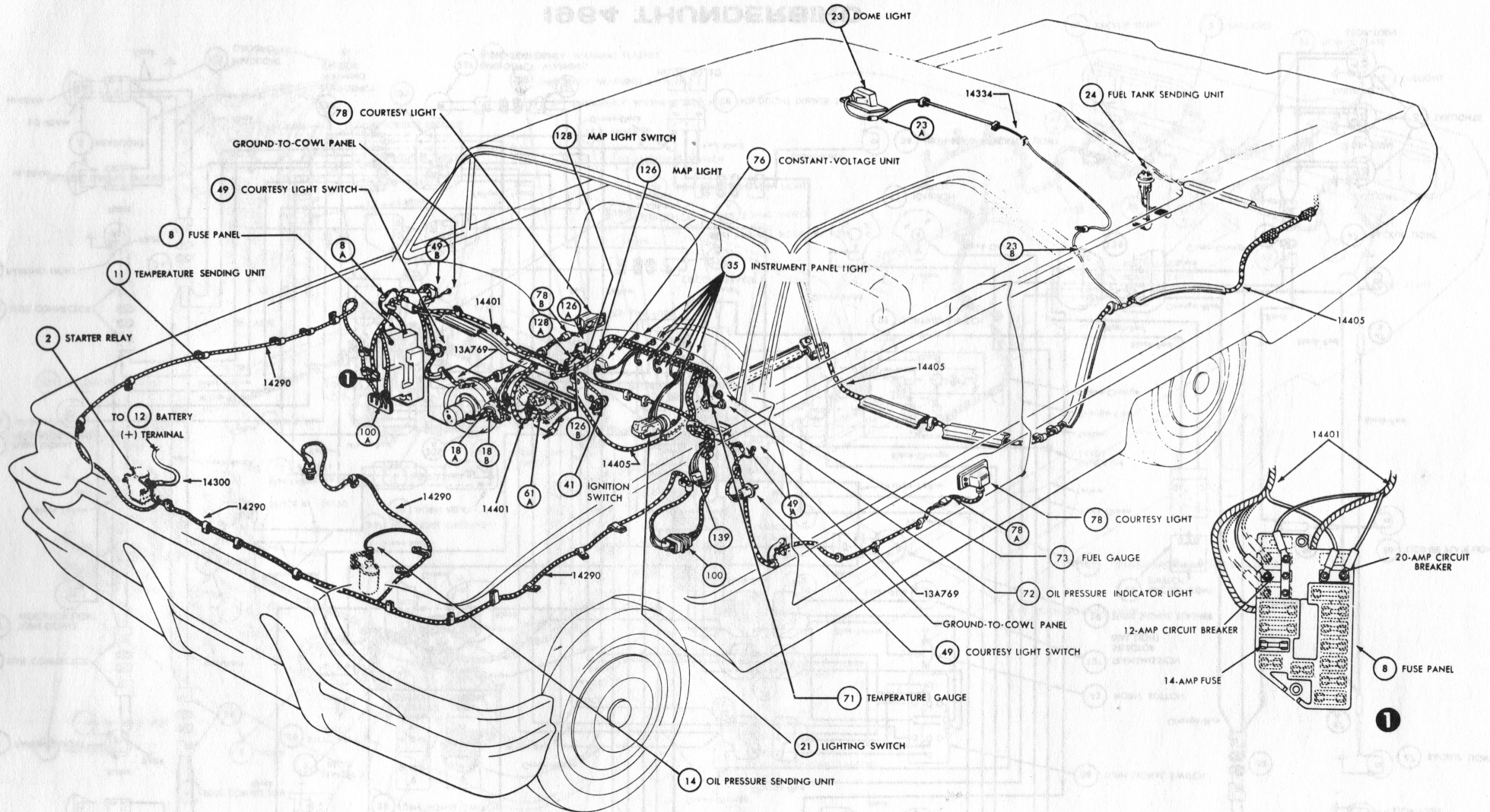
1964 THUNDERBIRD INTERIOR LIGHTING, WINDSHIELD WIPER AND GAUGE WIRING
