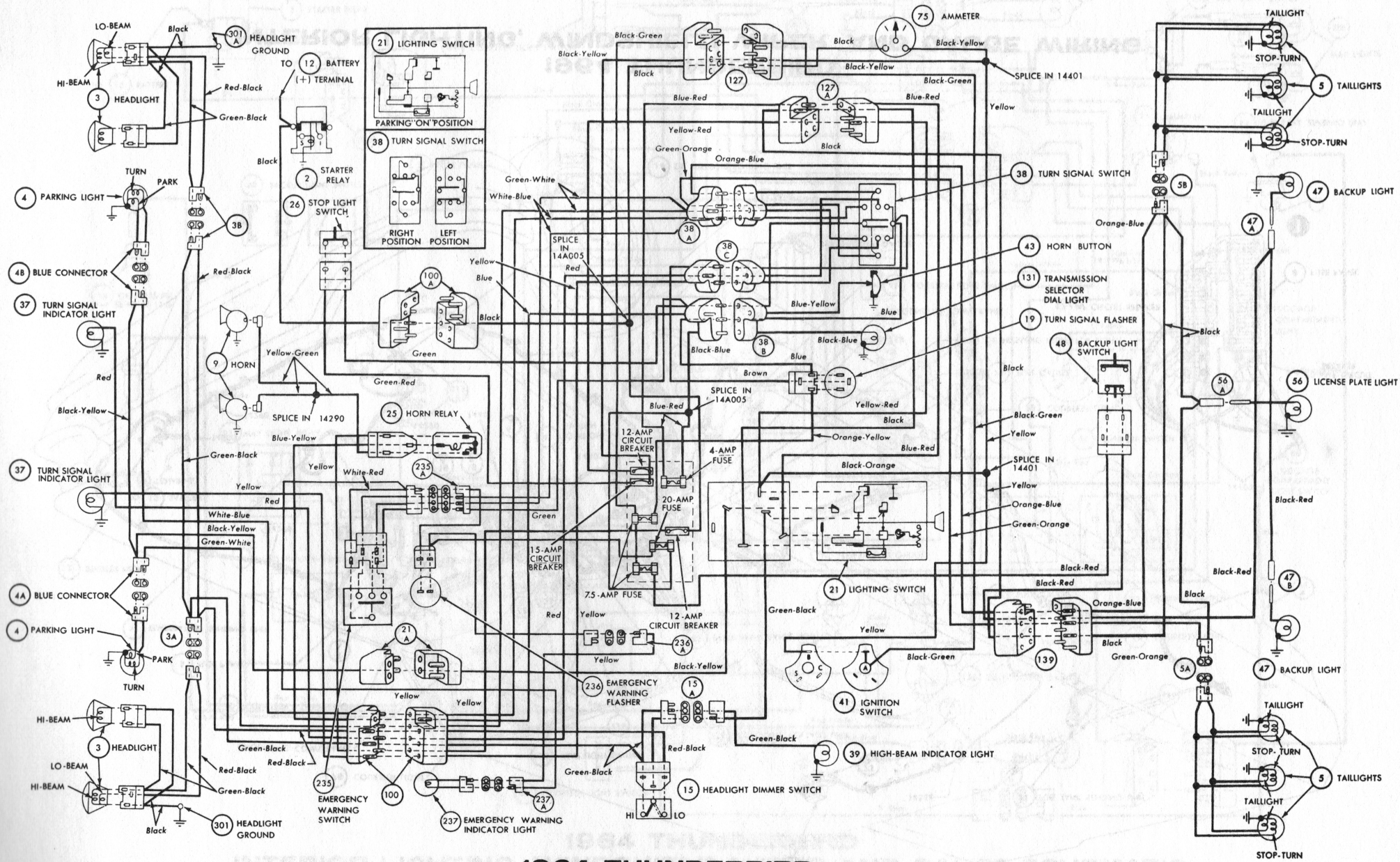
1964 THUNDERBIRD EXTERIOR LIGHTING, TURN SIGNALS AND HORN SCHEMATIC
