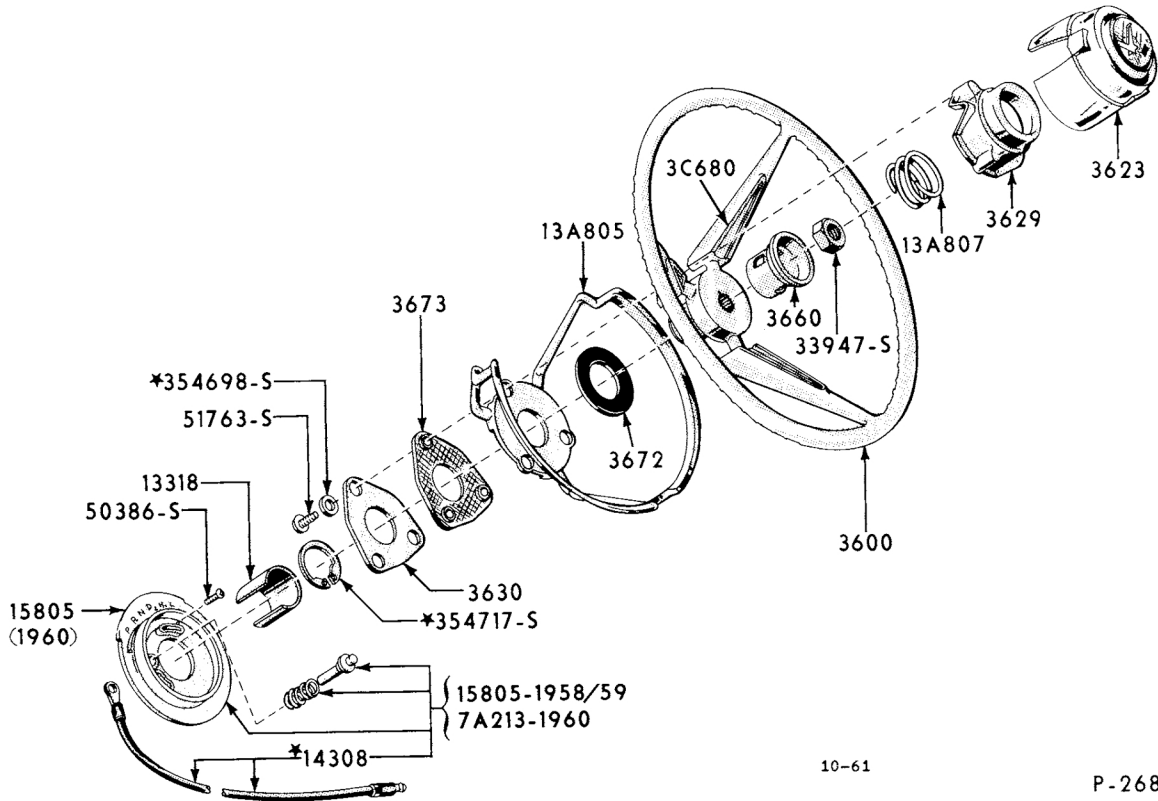
1958-1960 THUNDERBIRD STEERING WHEEL & HORN RING
